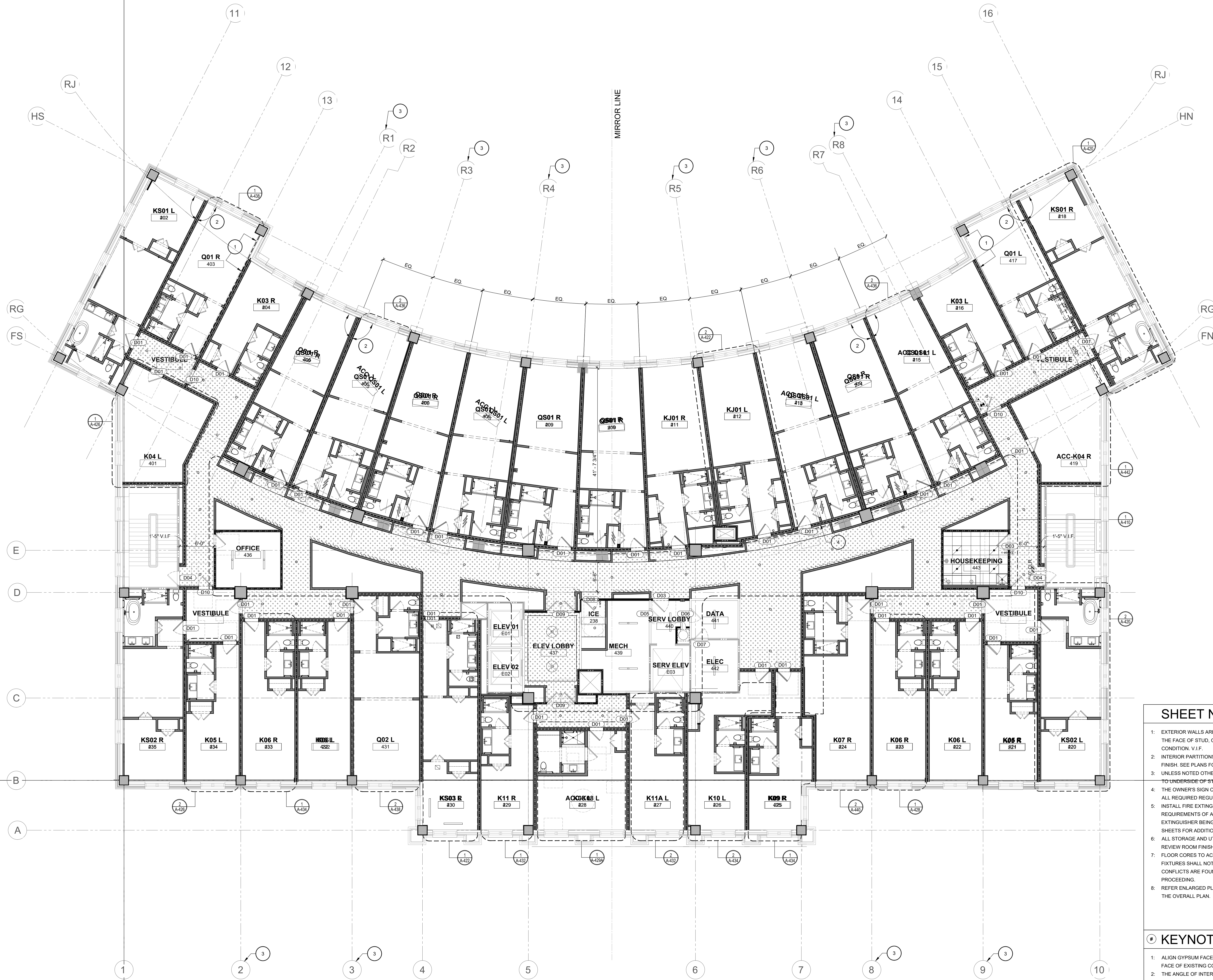
1 OVERALL FLOOR PLAN - 4TH FLOOR SCALE: 1/8" = 1'-0"
