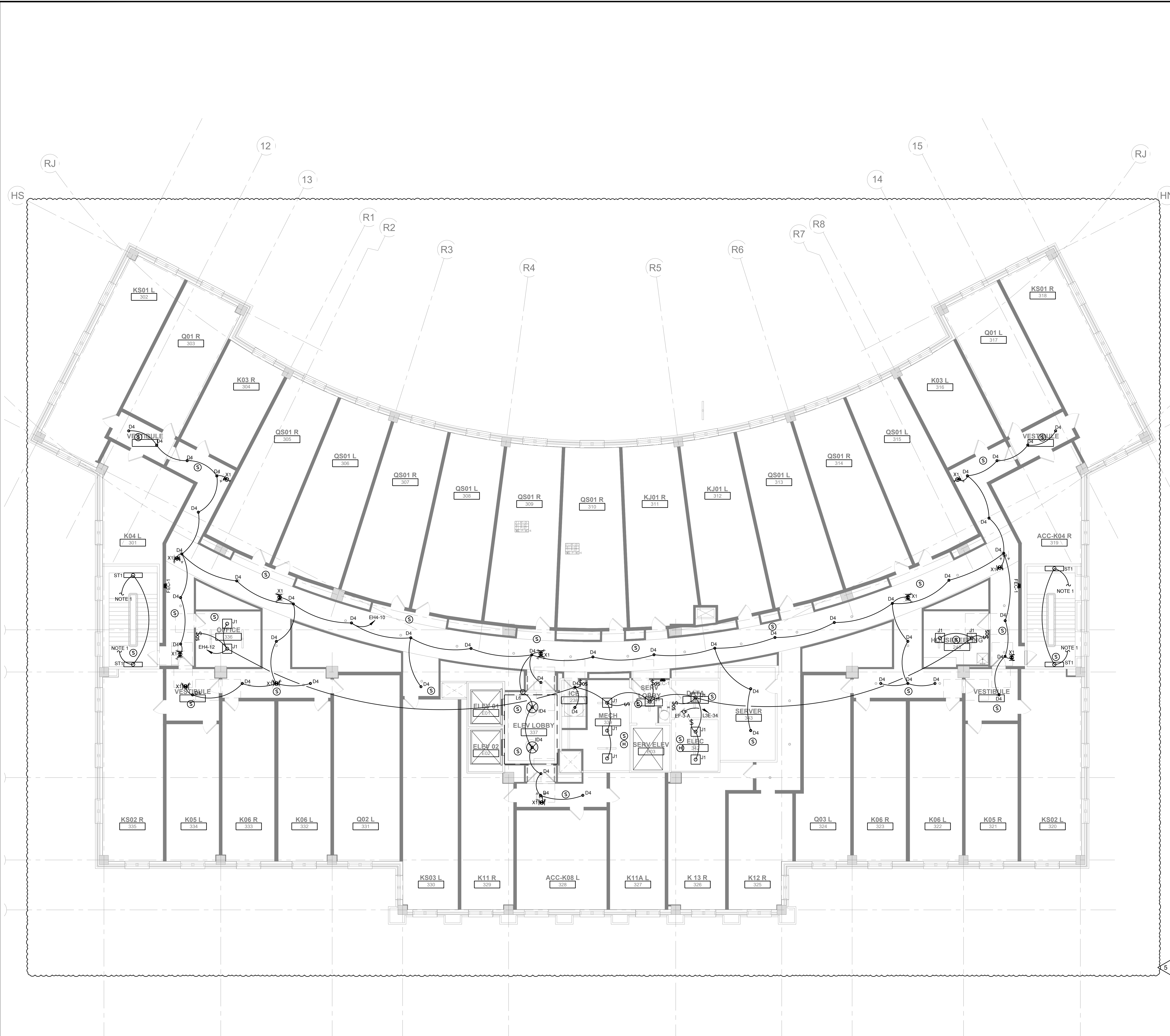
1 ELECTRICAL OVERALL CEILING PLAN - LEVEL 3 SCALE: 1/8" = 1'-0"
