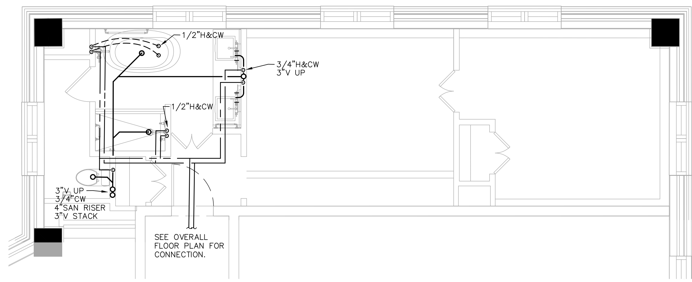
1 KS01 L Typical Guestroom Plan SCALE: 1/4" = 1'-0"
