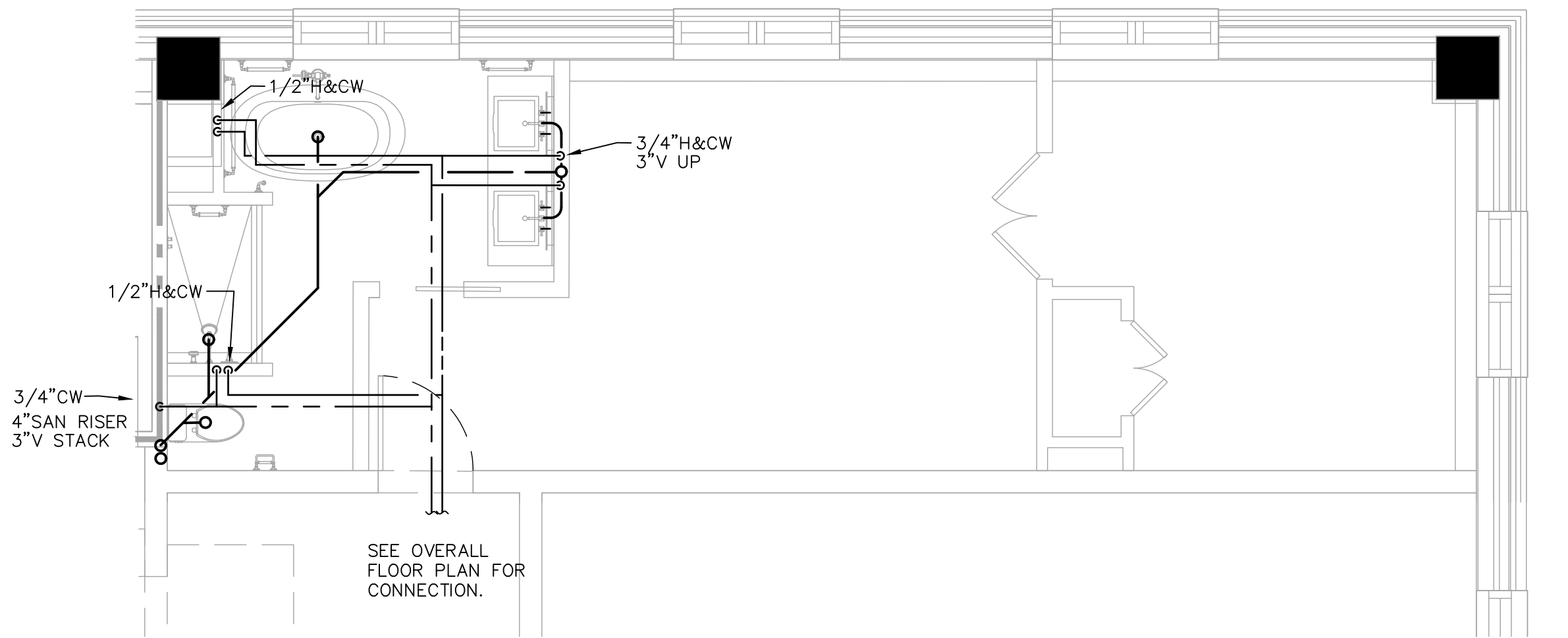
3 KS02 L Typical Guestroom Plan SCALE: 1/4" = 1'-0"
