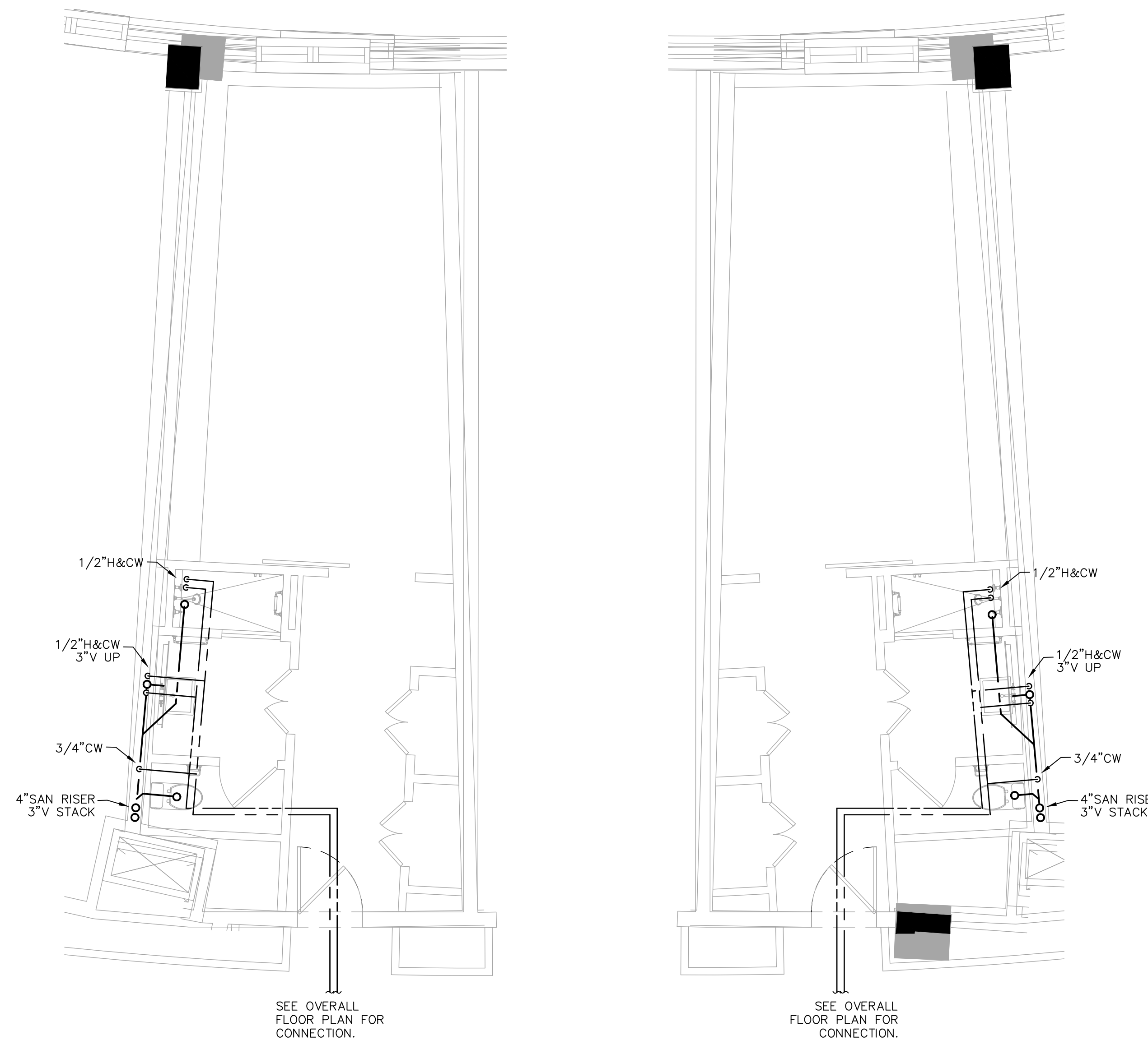
5 KJ01 L Typical Guestroom Plan SCALE: 1/4" = 1'-0"
