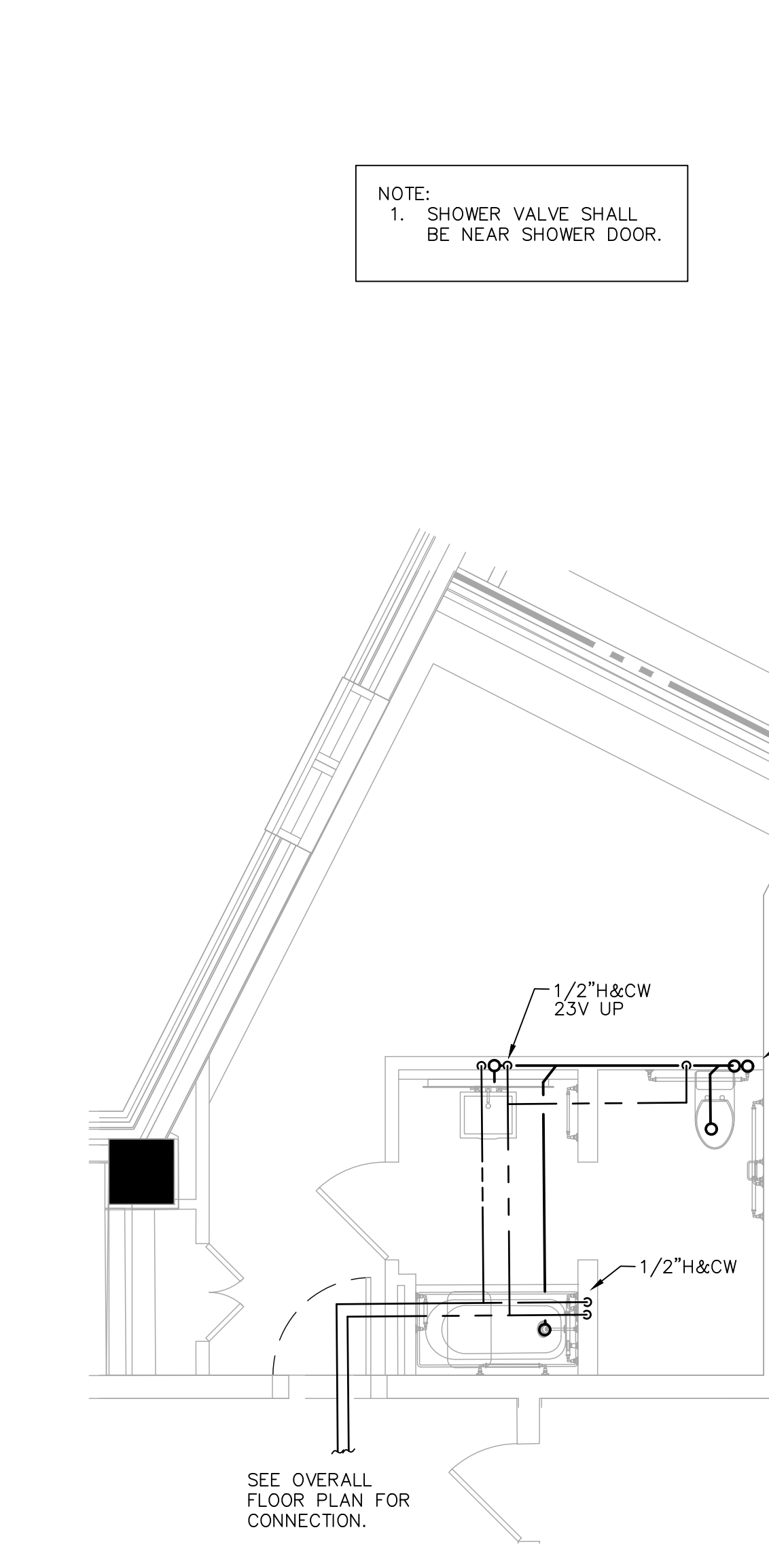
9 ACC K04 R Typical Guestroom Plan SCALE: 1/4" = 1'-0"
