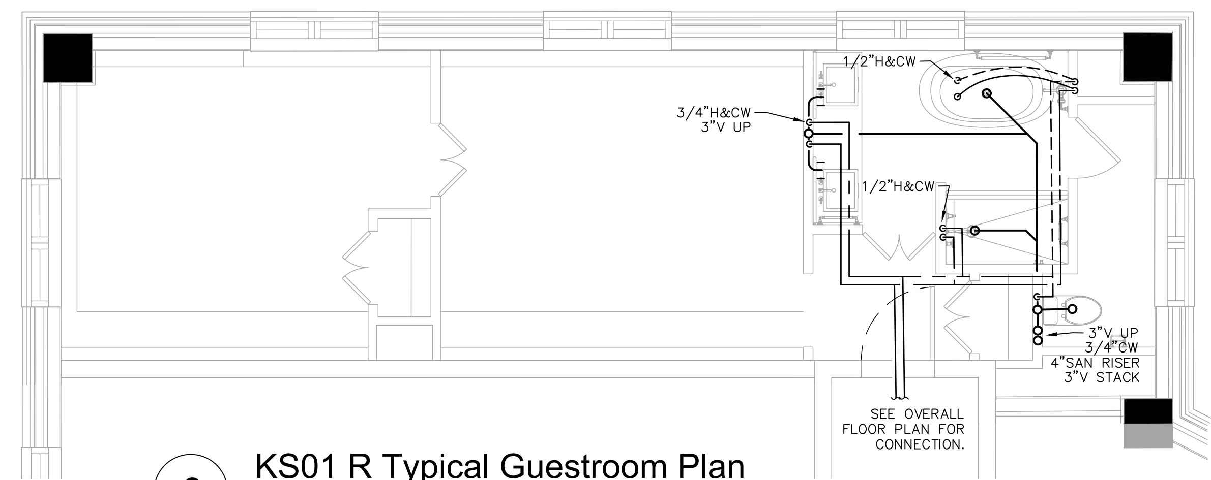
2 KS01 R Typical Guestroom Plan SCALE: 1/4" = 1'-0"
