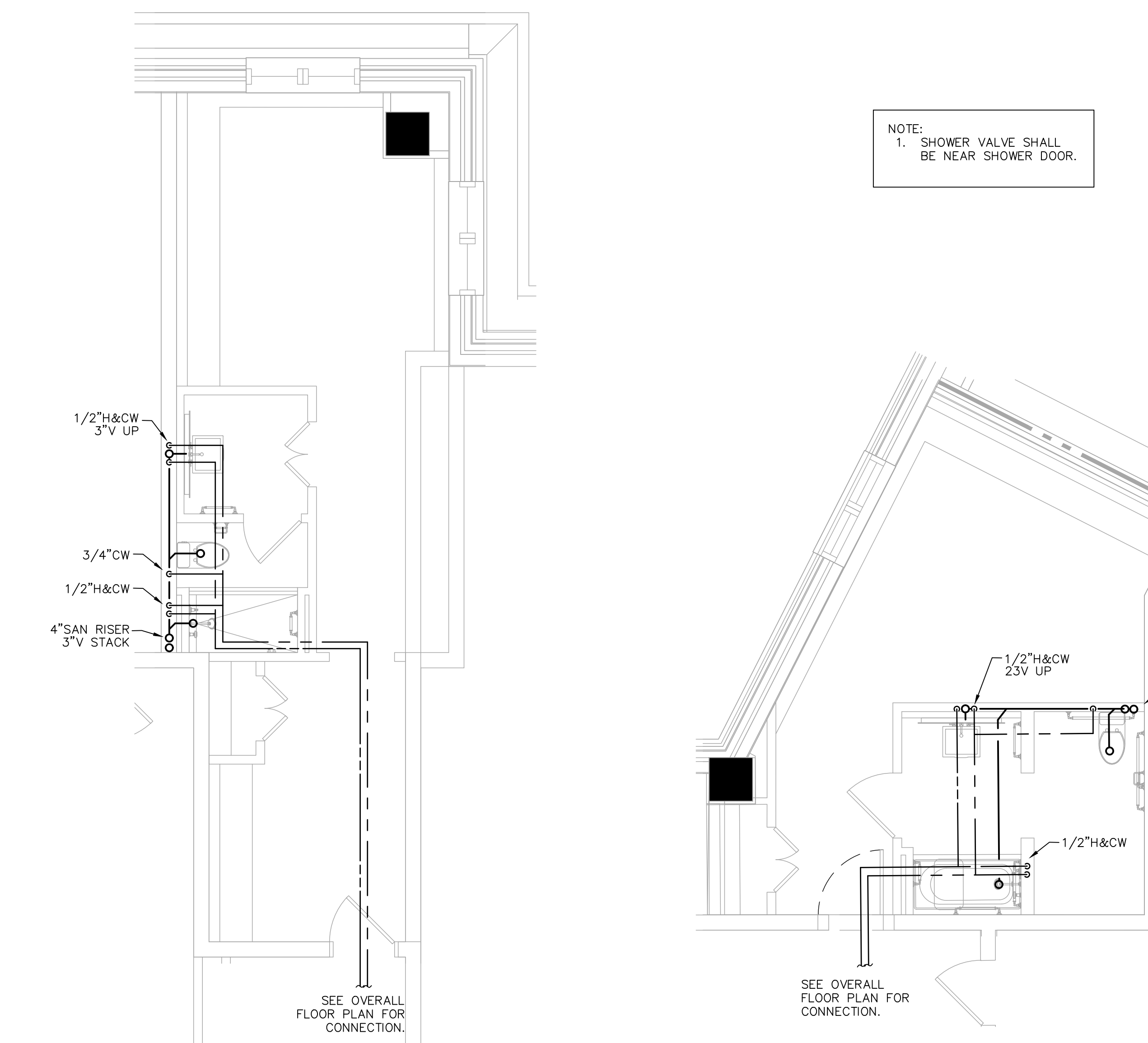
8 KJ02 R Typical Guestroom Plan SCALE: 1/4" = 1'-0"
