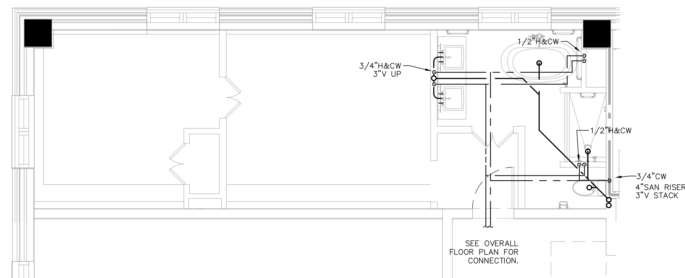
4 KS02 R Typical Guestroom Plan SCALE: 1/4" = 1'-0"
